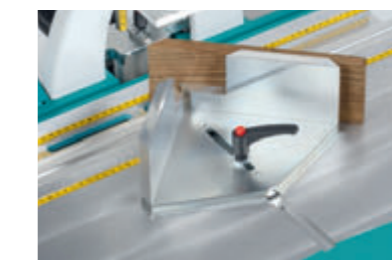
Angle fence plate elevation
